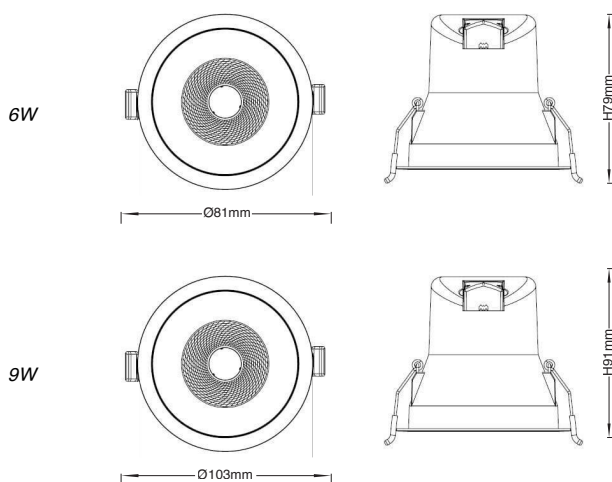
Misa Dimensions(mm)-
