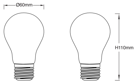
Lifey Dimensions(mm)-
