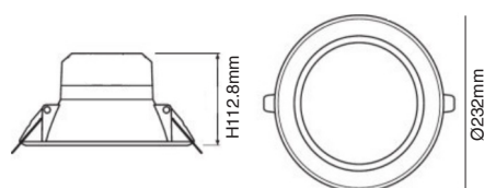
Axton Dimensions(mm)
